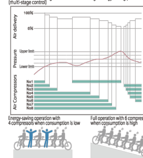
Operation of multi-stage control to achieve high energy-saving performance (multi-stage control)
