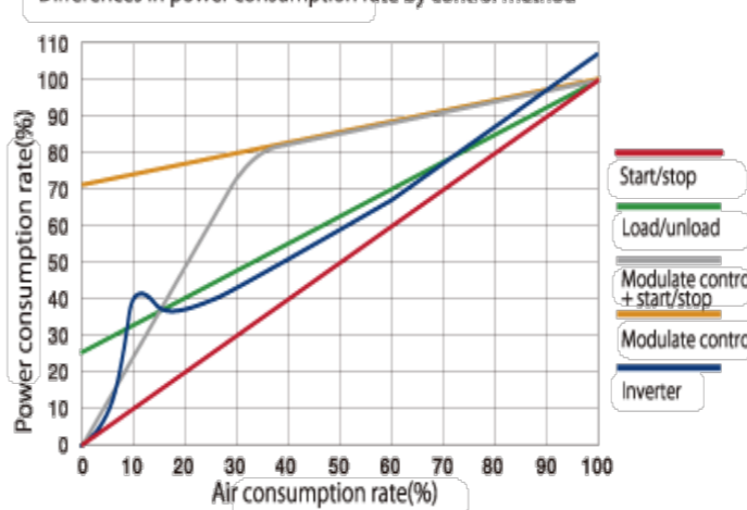
Operation of multi-stage control to achieve high energy-saving performance (multi-stage control)
